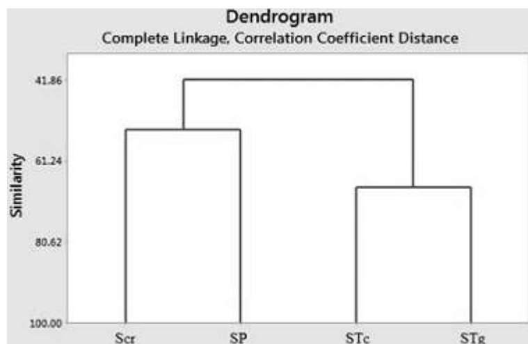
Figure 6. Dendrogram of biochemical parameters for control group.
