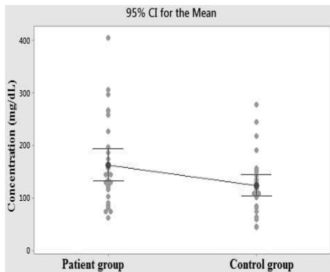
Figure 2. Interval plot of SP concentration for patient and control groups with a diagonal line connecting the means
