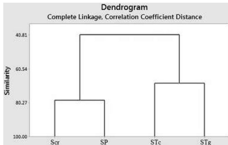
Figure 5. Dendrogram of biochemicals for patient group.
