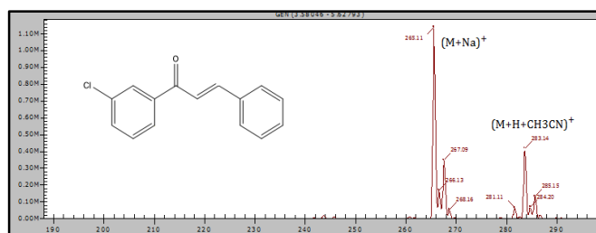
Figure 6 LC-MS spectrum of (E)-1-(3-chlorophenyl)-3-phenylprop-2-en-1-one
