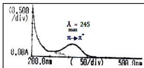
Figure 3. UV-visible spectrum of (E)-1-(3-chlorophenyl)-3-phenylprop-2-en-1-one (I)
