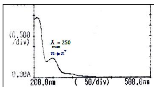
Figure (10) UV-visible spectrum of (E)-1,3-bis(3-chlorophenyl) prop-2-en-1-one (III)
