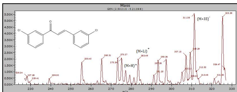
Figure(11) LC-MS spectrum of (E)-1,3-bis(3-chlorophenyl) prop-2-en-1-one (III)
