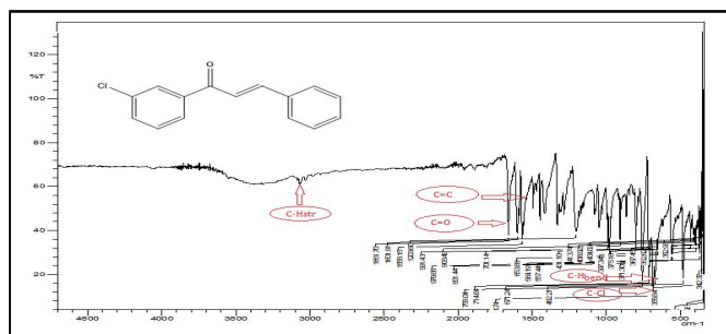
Figure 2 Infra-red (IR) spectrum of (E)-1-(3-chlorophenyl)-3-phenylprop-2-en-1-one (I)
