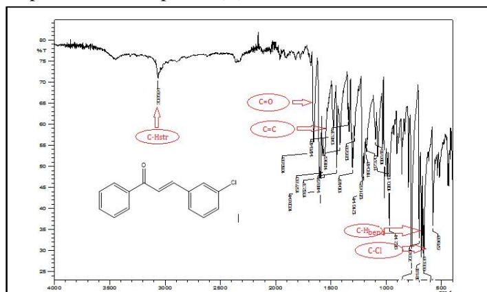
Figure 7 Infra-red (IR) spectrum of (E)-3-(3-chlorophenyl)-1-phenylprop-2-en-1-one
