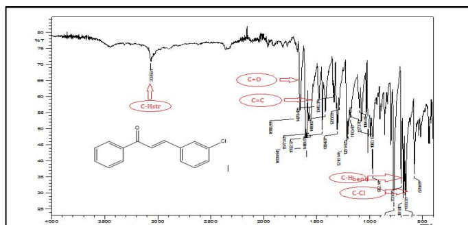
Figure 5 Infra-red (IR) spectrum of (E)-3-(3-chlorophenyl)-1-phenylprop-2-en-1-one
